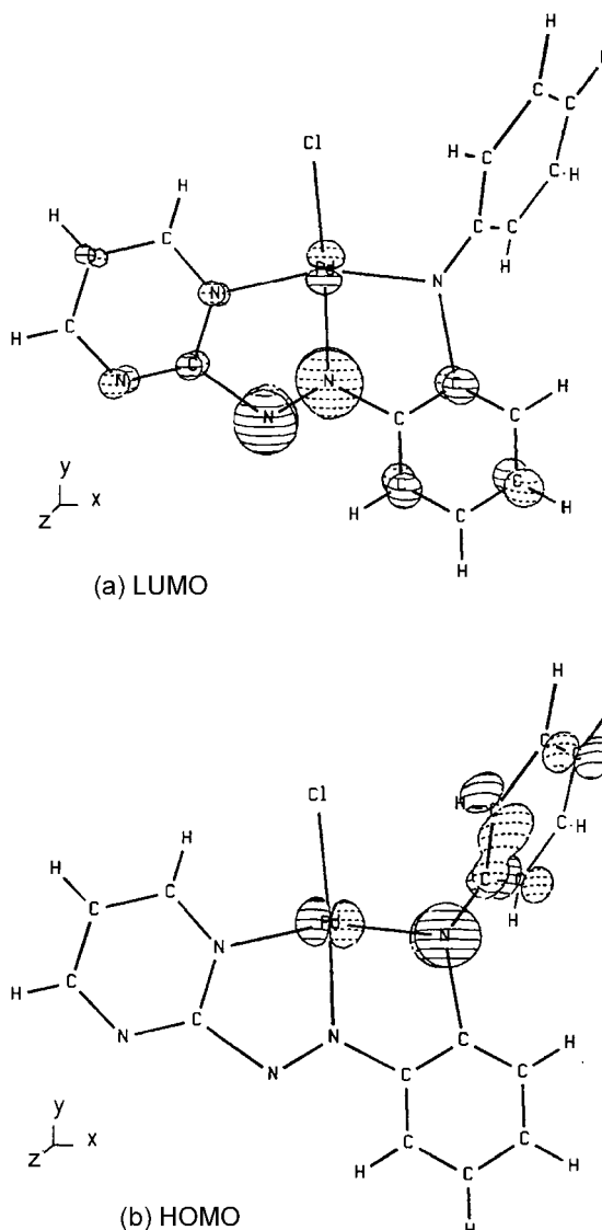
Figure 6. LUMO and HOMO of \text{Pd}(\text{papm-}N\text{-C}_6\text{H}_5)\text{Cl}
