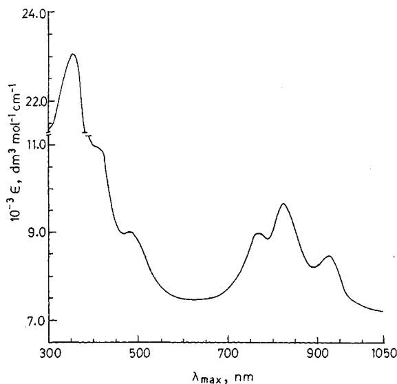
Figure 1. Electronic spectra of \text{Pd(papm-N-OCH}_3\text{-}p\text{)Cl} ( 5a ) in \text{CHCl}_3
