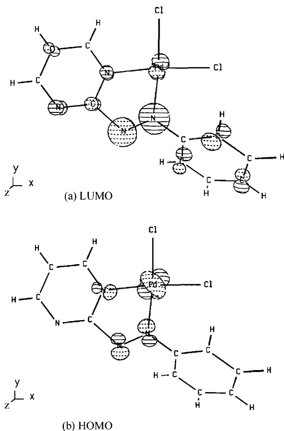
Figure 5. LUMO and HOMO of \text{Pd}(\text{papm})\text{Cl}_2
